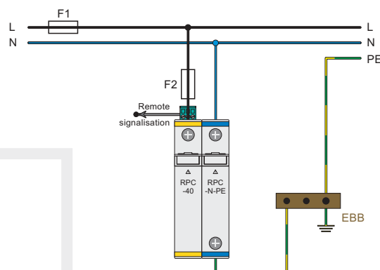
TT (1+1) single-phase network
