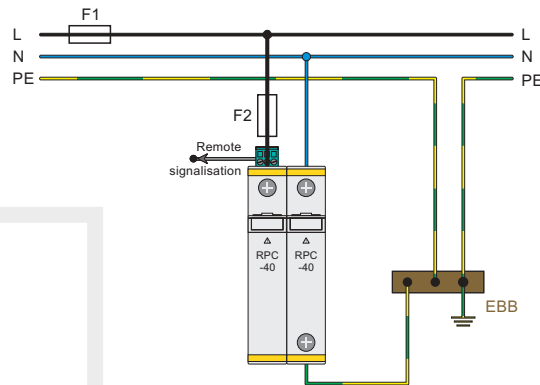
TNS / TNC (2+0) single-phase network
